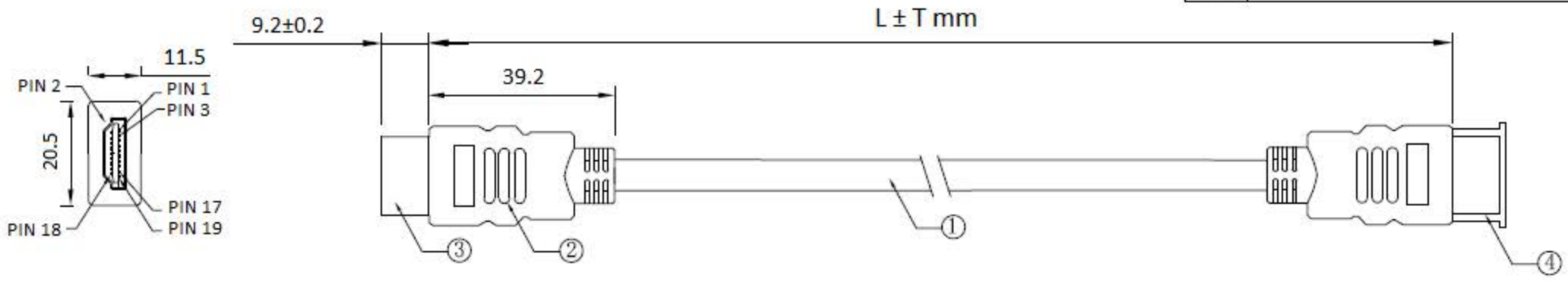
Pin Assignment
